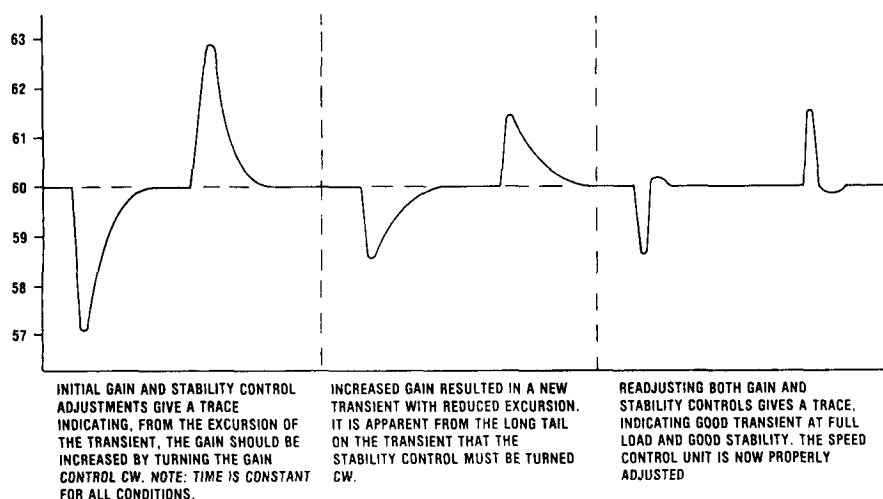
Figure 4. Typical performance chart
