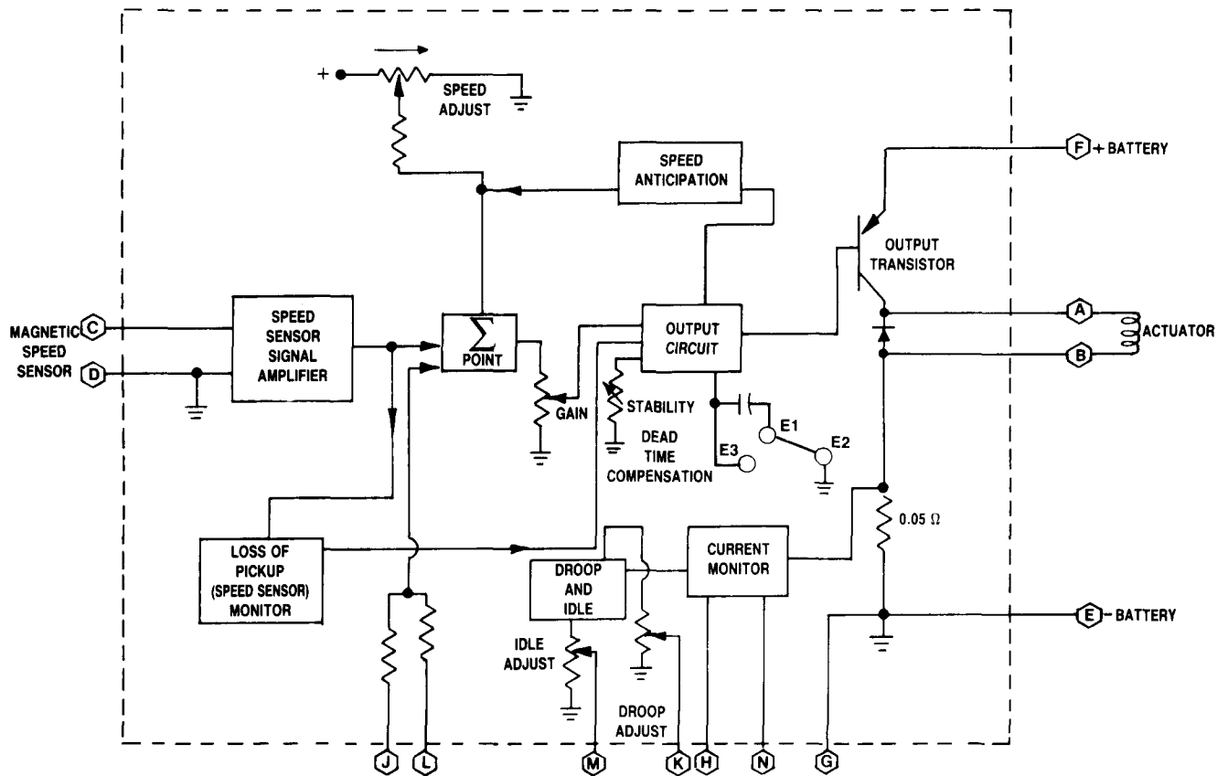
Figure 2. Functional schematic
